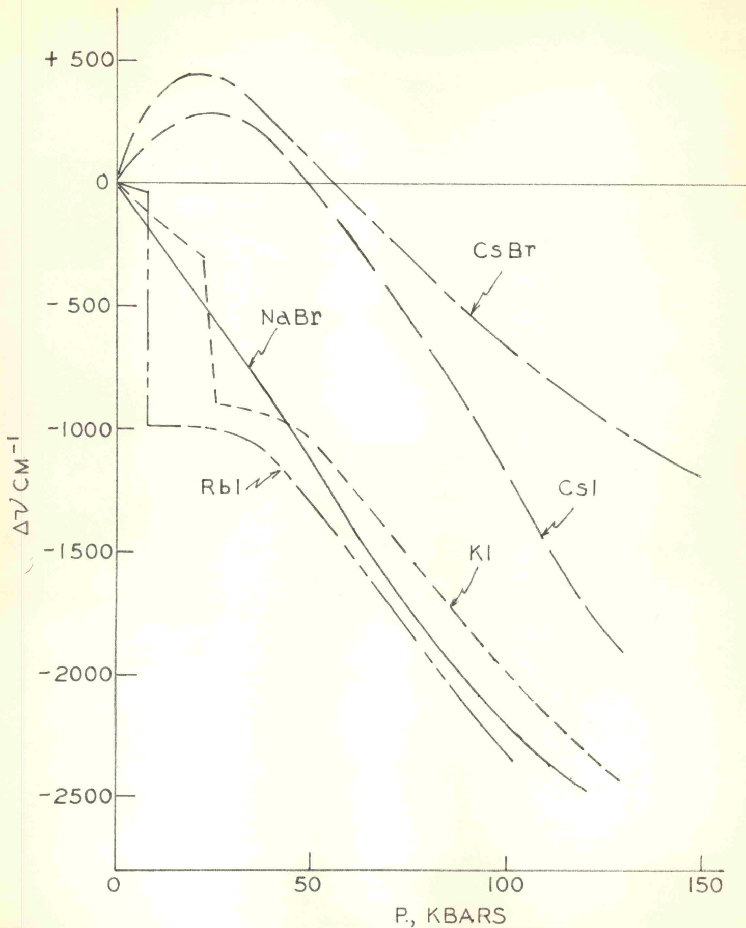
FIG.3 \Delta\nu VS. PRESSURE \text{Ti}^+ IN ALKALI HALIDES
